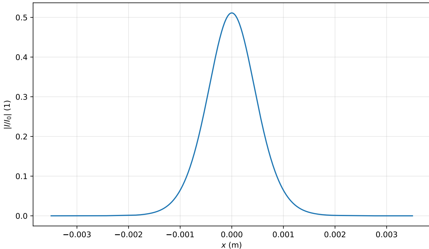
Intensity profile I(x, y = 0, z = 3.264m)/I_0 , P_{in}=0.5P_{cr} , artificial time
